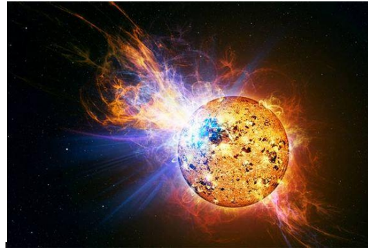
A powerful flare that erupted from the red dwarf star EV Lacertae www.space.com
