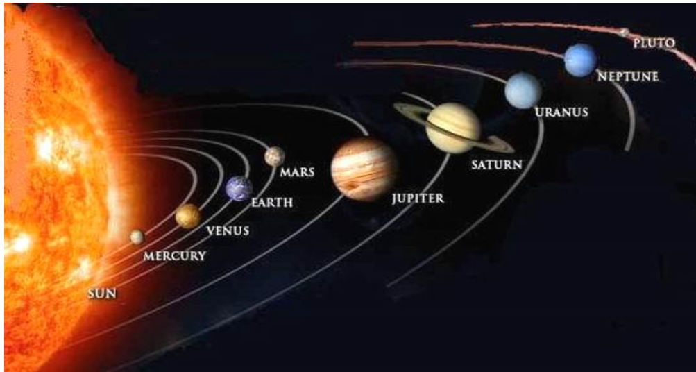
Our Cosmic Neighborhood and beyond the Cosmic Web
